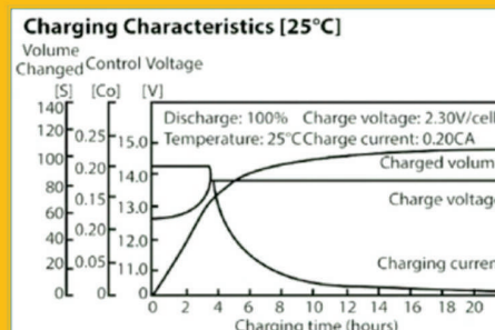
Charging Characteristics
