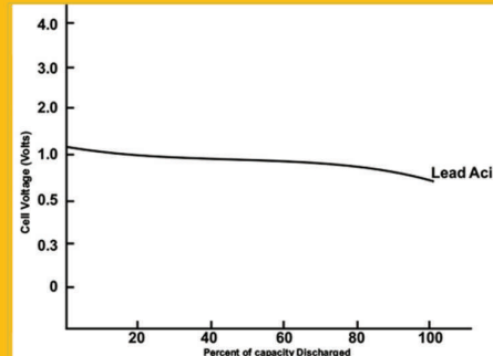
Discharging Characteristics
