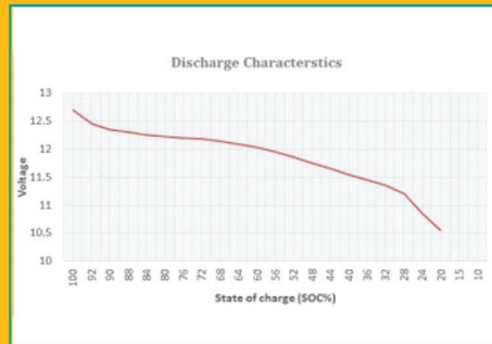
Discharging Characteristics
