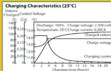
Charging Characteristics
