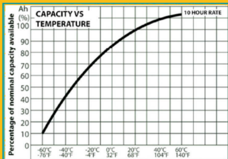
Capacity vs Temperature
